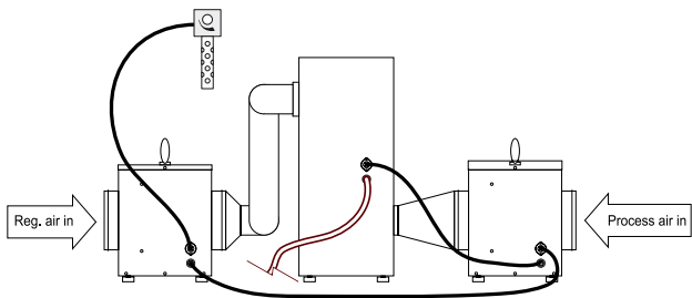
Example of two pressure boxes connected to two inlets to push the air through the unit.
