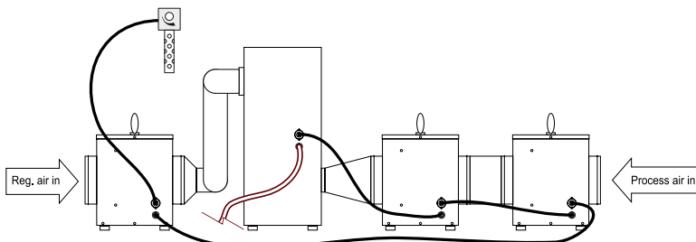
Example of three pressure boxes connected to two inlets to push the air through the unit.
