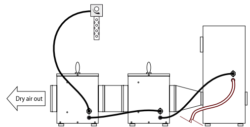
Example of two pressure boxes connected to one outlet to pull air through the unit.
